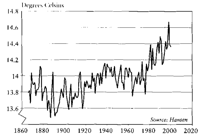
Figure 2-3. Average Temperature at the Earth's Surface, 1866–2000
