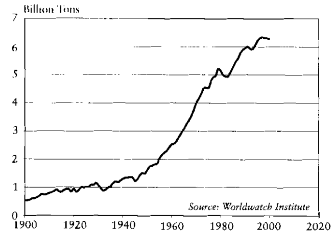
Figure 2-1. World Carbon Emissions from Fossil Fuel Burning, 1900–2000
